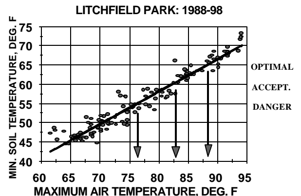
Fig. 2. Minimum soil vs. maximum air temperature for Litchfield Park. Arrows indicate maximum temperatures associated with critical temperature thresholds for germination.
