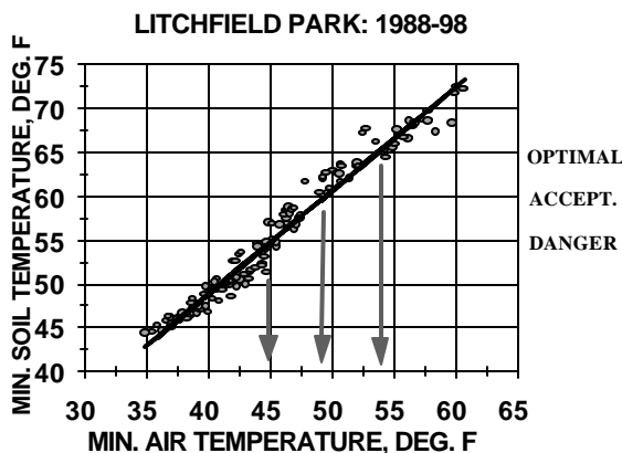
Fig. 1. Minimum soil vs. minimum air temperature for Litchfield Park. Arrows indicate minimum temperatures associated with critical temperature thresholds for germination.
