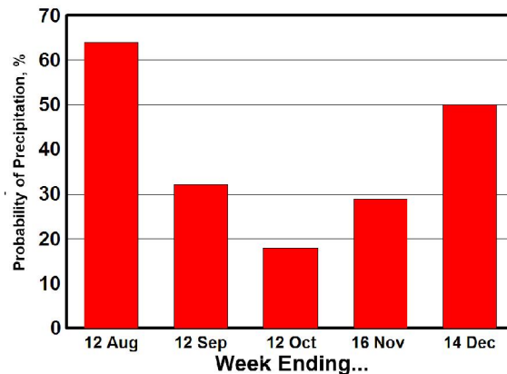
Figure 1. Probability of precipitation for selected weeks at the AZMET weather station located near Coolidge, AZ.
