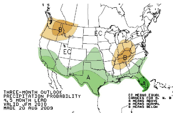
Figure 2. Precipitation forecast for the period 1 Jan. through 31 Mar. 2010. Forecasting models indicate a bias toward above normal precipitation in areas shaded in green. Source: NOAA Climate Prediction Center: http://www.cpc.noaa.gov/products/predictions/long_range/ .
